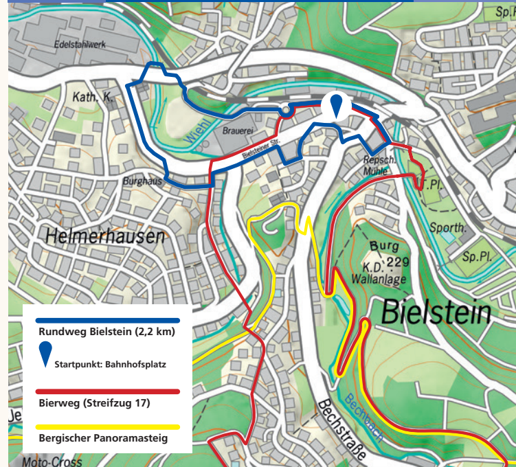
Burghaus (Brandt, 2012)
